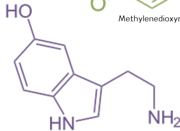
Serotonin
