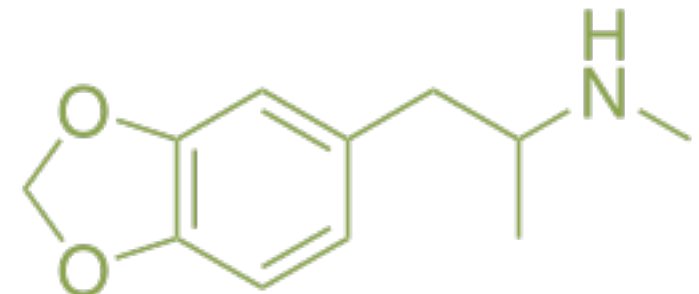
Methylendioxyamphetamine
