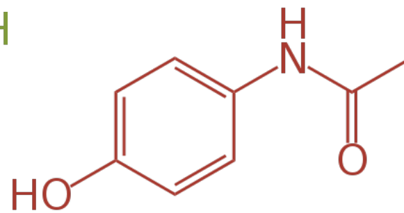
Acetaminophen
