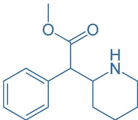
Methylphenidate
