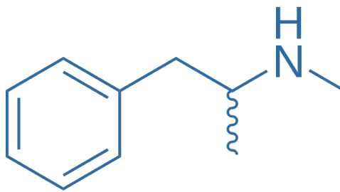
Methamphetamine
